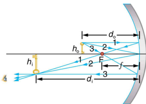
Figure 25.7.4: A case 1 image for a mirror. An object is farther from the converging mirror than its focal length. Rays from a common point on the object are traced using the rules in the text. Ray 1 approaches parallel to the axis, ray 2 strikes the center of the mirror, and ray 3 goes through the focal point on the way toward the mirror. All three rays cross at the same point after being reflected, locating the inverted real image. Although three rays are shown, only two of the three are needed to locate the image and determine its height.
